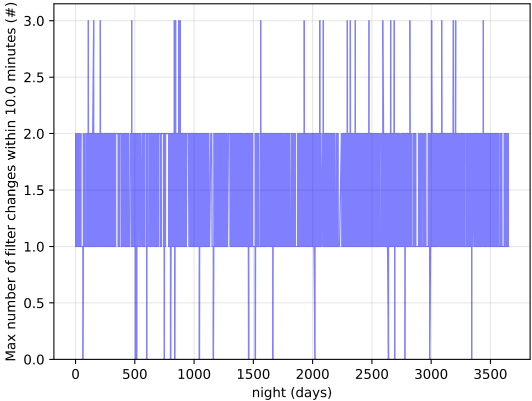
roll_uniform_early_half_accordion1_mjdp0_v3.4_10yrs Per Night: Max number of filter changes within 10.0 minutes
