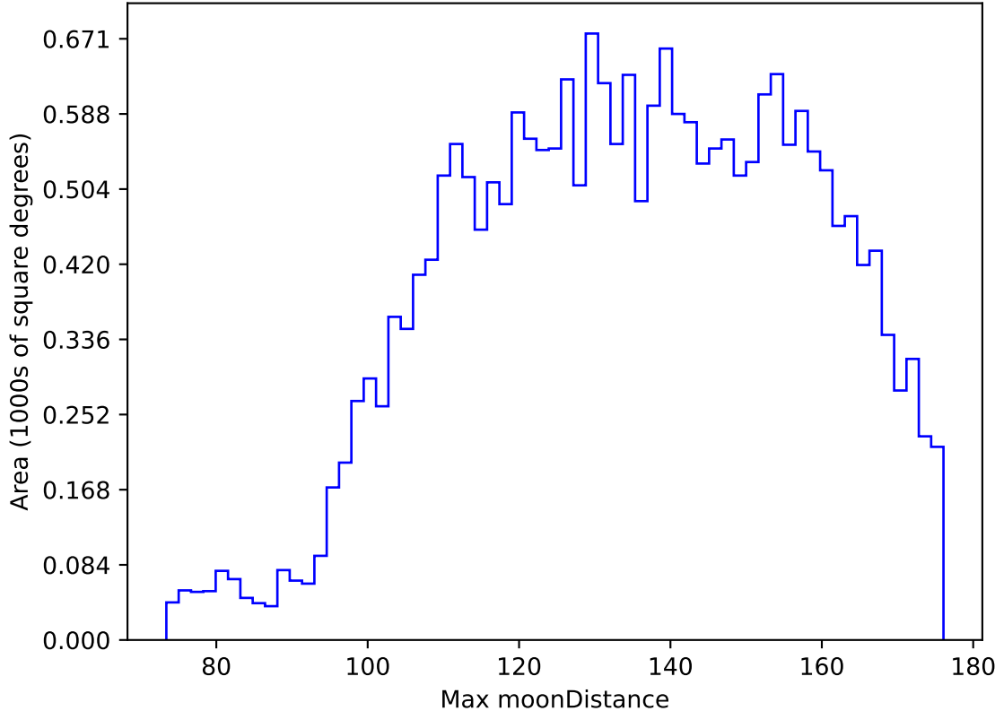
roll_uniform_early_half_accordion1_mjdp0_v3.4_10yrs All sky y band: Max moonDistance
