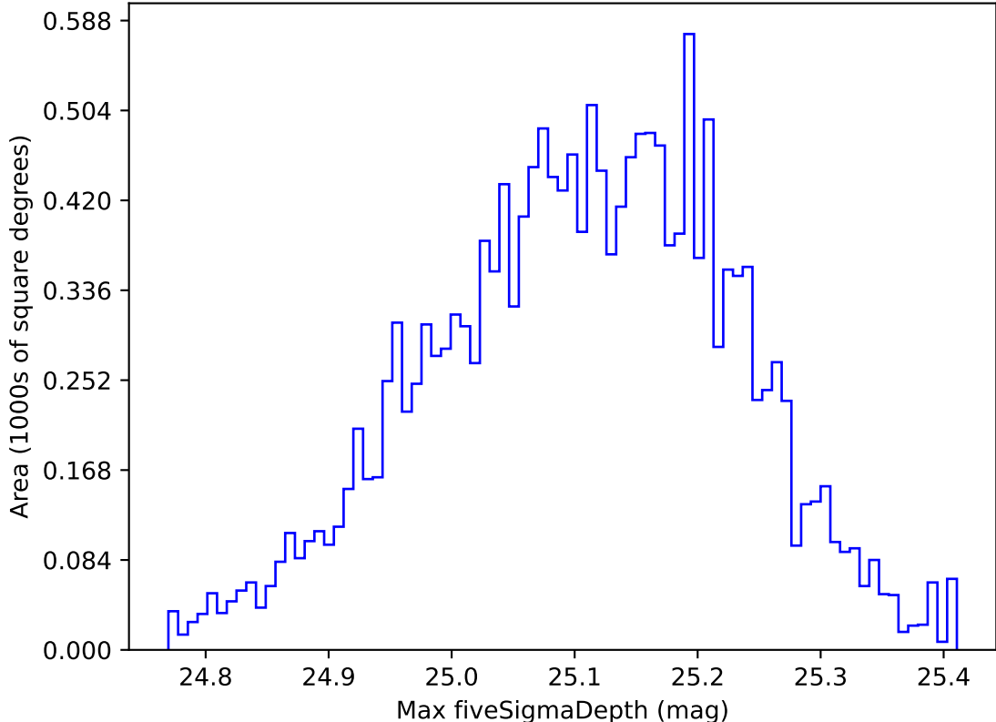
roll_uniform_early_half_accordion1_mjdp0_v3.4_10yrs WFD g band: Max fiveSigmaDepth
