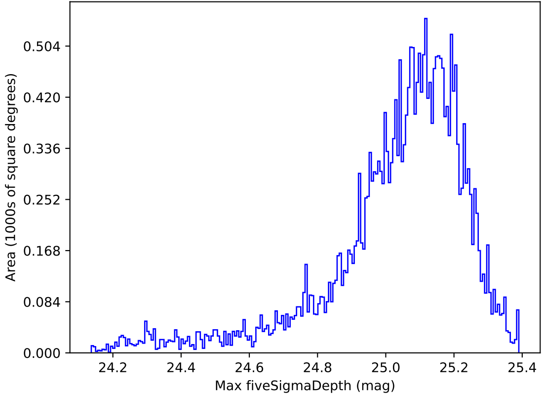
roll_uniform_early_half_accordion1_mjdp0_v3.4_10yrs All sky all bands: Max fiveSigmaDepth
