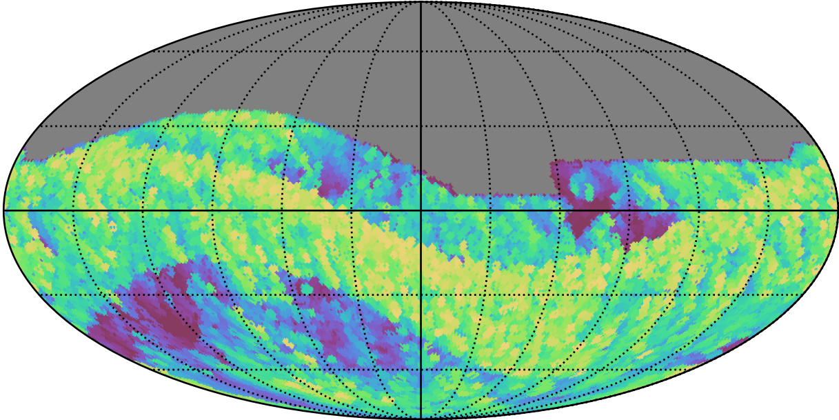
roll_uniform_early_half_accordion1_mjdp0_v3.4_10yrs All sky i band: Max airmass
