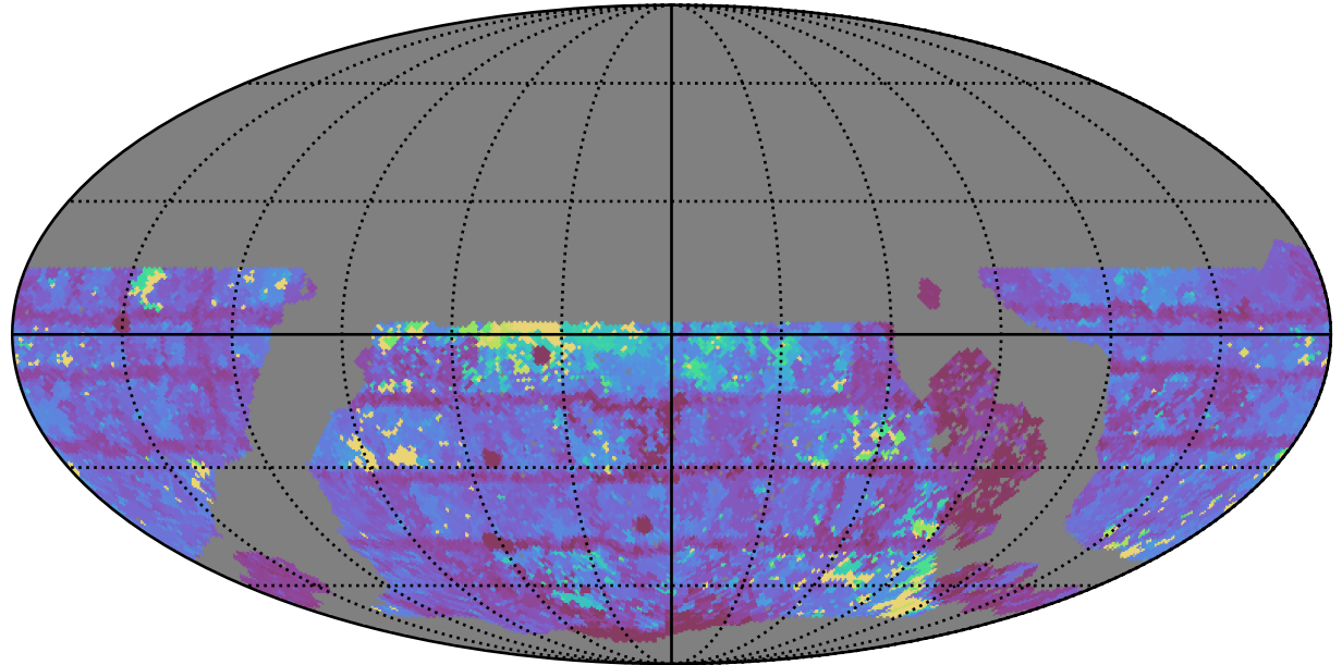
roll_uniform_early_half_accordion1_mjdp0_v3.4_10yrs WFD z band: Max Inter-Night Gap
