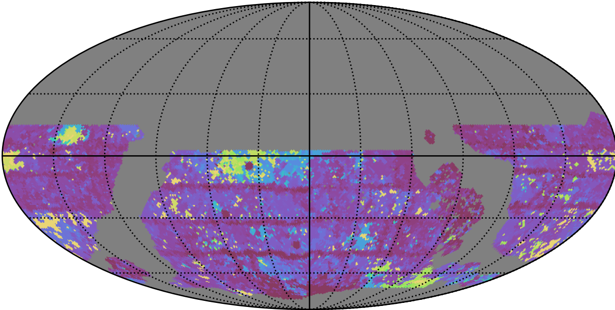
roll_uniform_early_half_accordion1_mjdp0_v3.4_10yrs WFD y band: Max Inter-Night Gap
