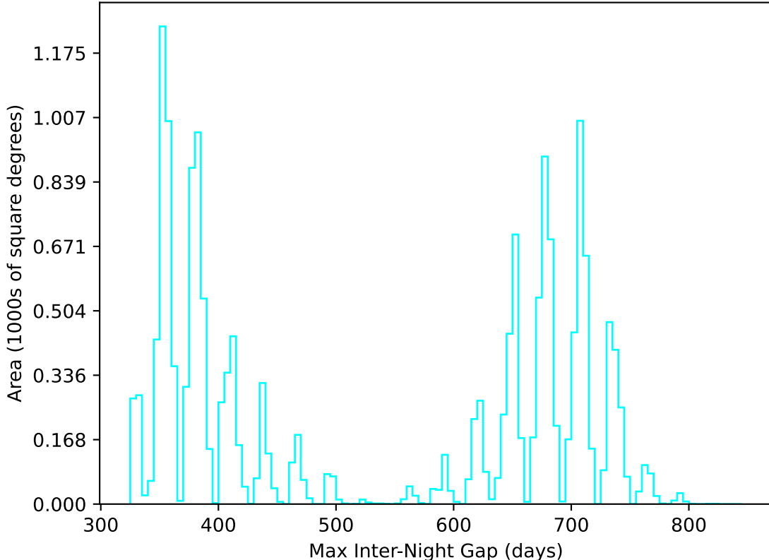
roll_uniform_early_half_accordion1_mjdp0_v3.4_10yrs WFD u band: Max Inter-Night Gap
