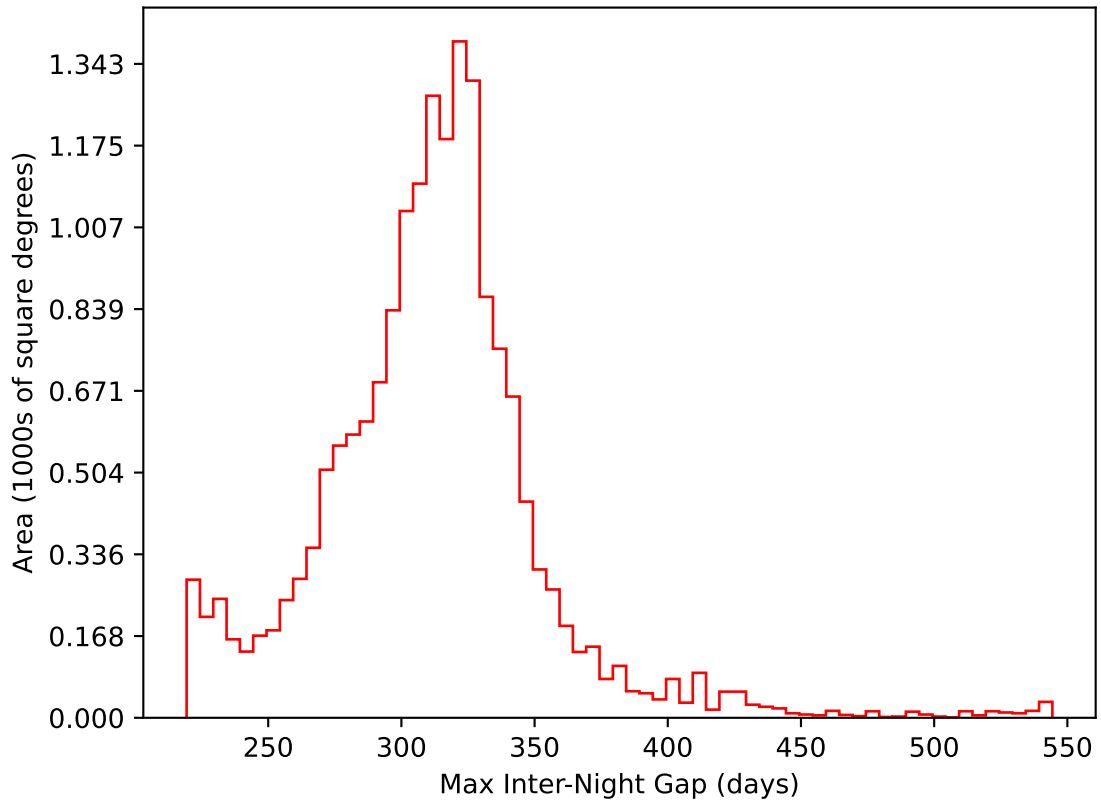
roll_uniform_early_half_accordion1_mjdp0_v3.4_10yrs WFD i band: Max Inter-Night Gap
