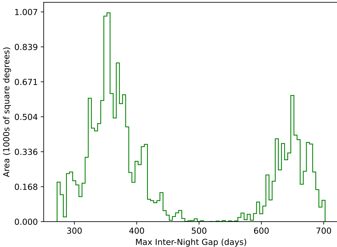
roll_uniform_early_half_accordion1_mjdp0_v3.4_10yrs WFD g band: Max Inter-Night Gap
