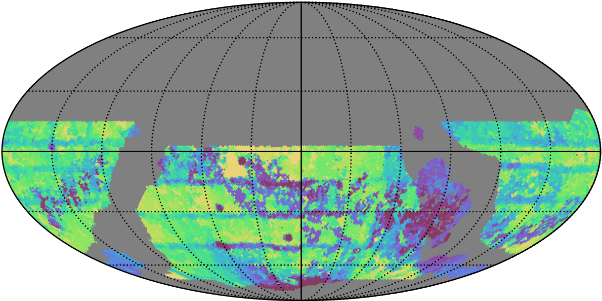
roll_uniform_early_half_accordion1_mjdp0_v3.4_10yrs WFD all bands: Max Inter-Night Gap
