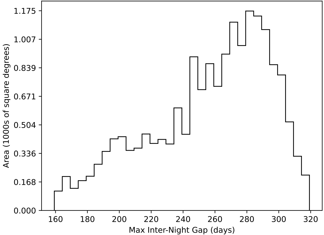
roll_uniform_early_half_accordion1_mjdp0_v3.4_10yrs WFD all bands: Max Inter-Night Gap
