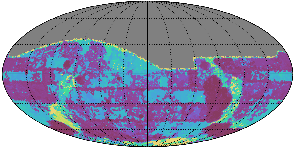
roll_uniform_early_half_accordion1_mjdp0_v3.4_10yrs All sky g band: Max Inter-Night Gap
