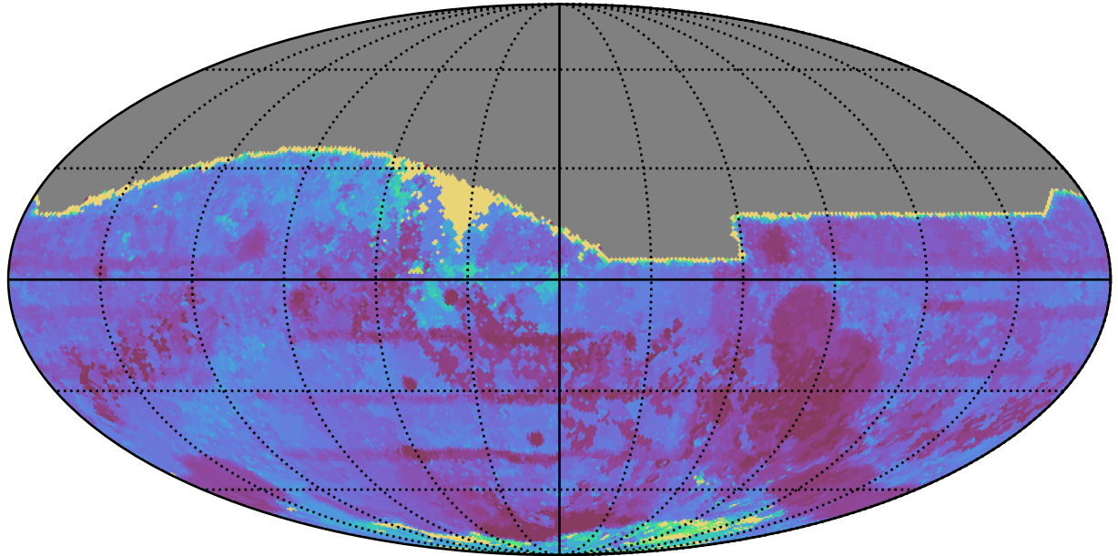
roll_uniform_early_half_accordion1_mjdp0_v3.4_10yrs All sky all bands: Max Inter-Night Gap
