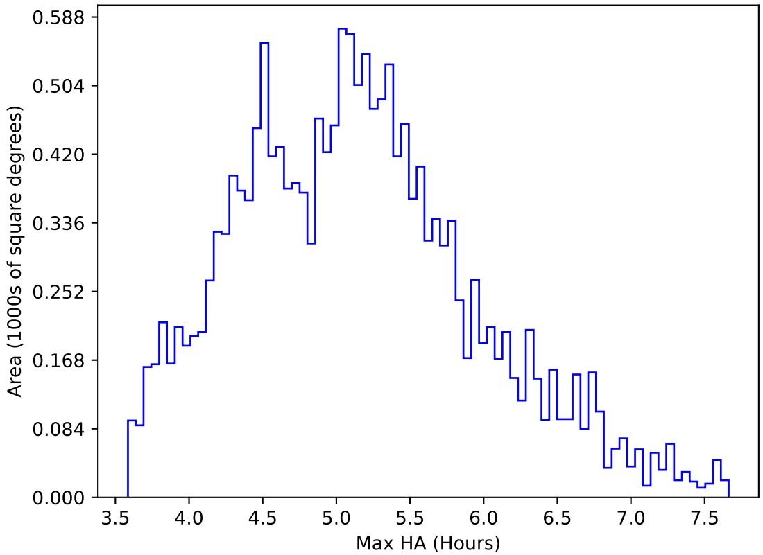
roll_uniform_early_half_accordion1_mjdp0_v3.4_10yrs WFD all bands: Max HA
