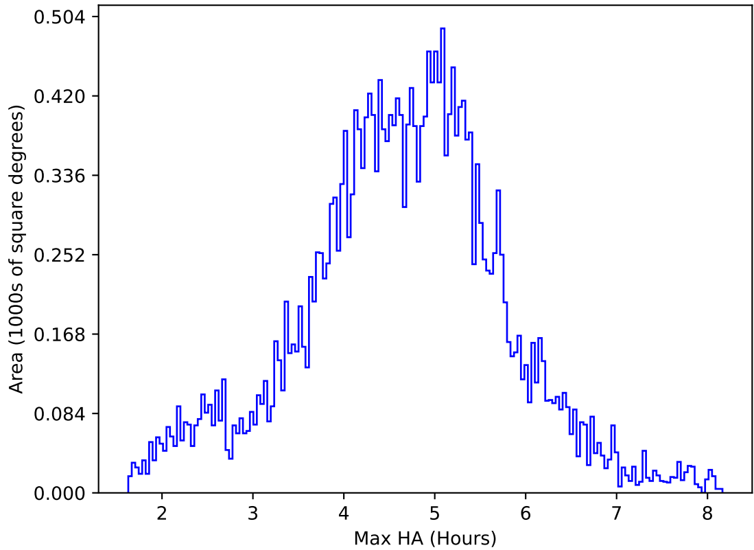
roll_uniform_early_half_accordion1_mjdp0_v3.4_10yrs All sky z band: Max HA
