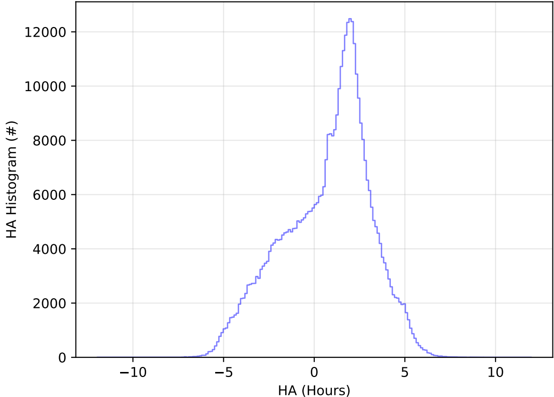
roll_uniform_early_half_accordion1_mjdp0_v3.4_10yrs WFD z band: HA Histogram
