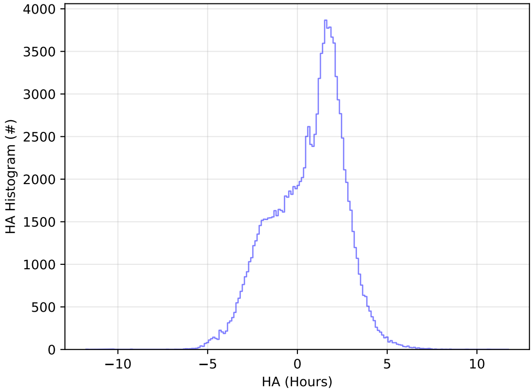
roll_uniform_early_half_accordion1_mjdp0_v3.4_10yrs WFD u band: HA Histogram
