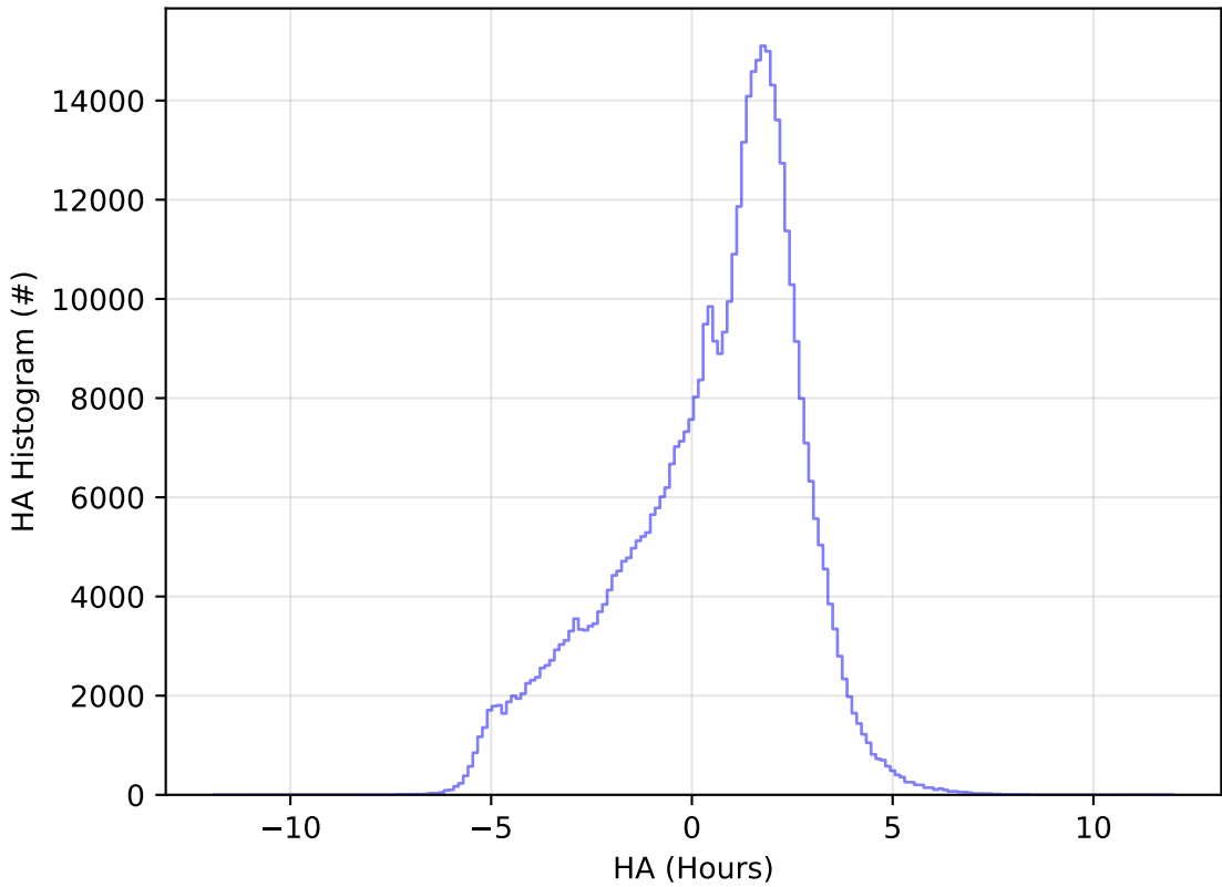
roll_uniform_early_half_accordion1_mjdp0_v3.4_10yrs WFD r band: HA Histogram
