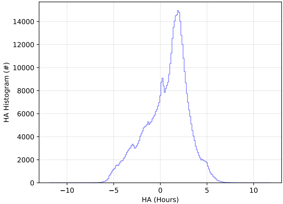
roll_uniform_early_half_accordion1_mjdp0_v3.4_10yrs WFD i band: HA Histogram
