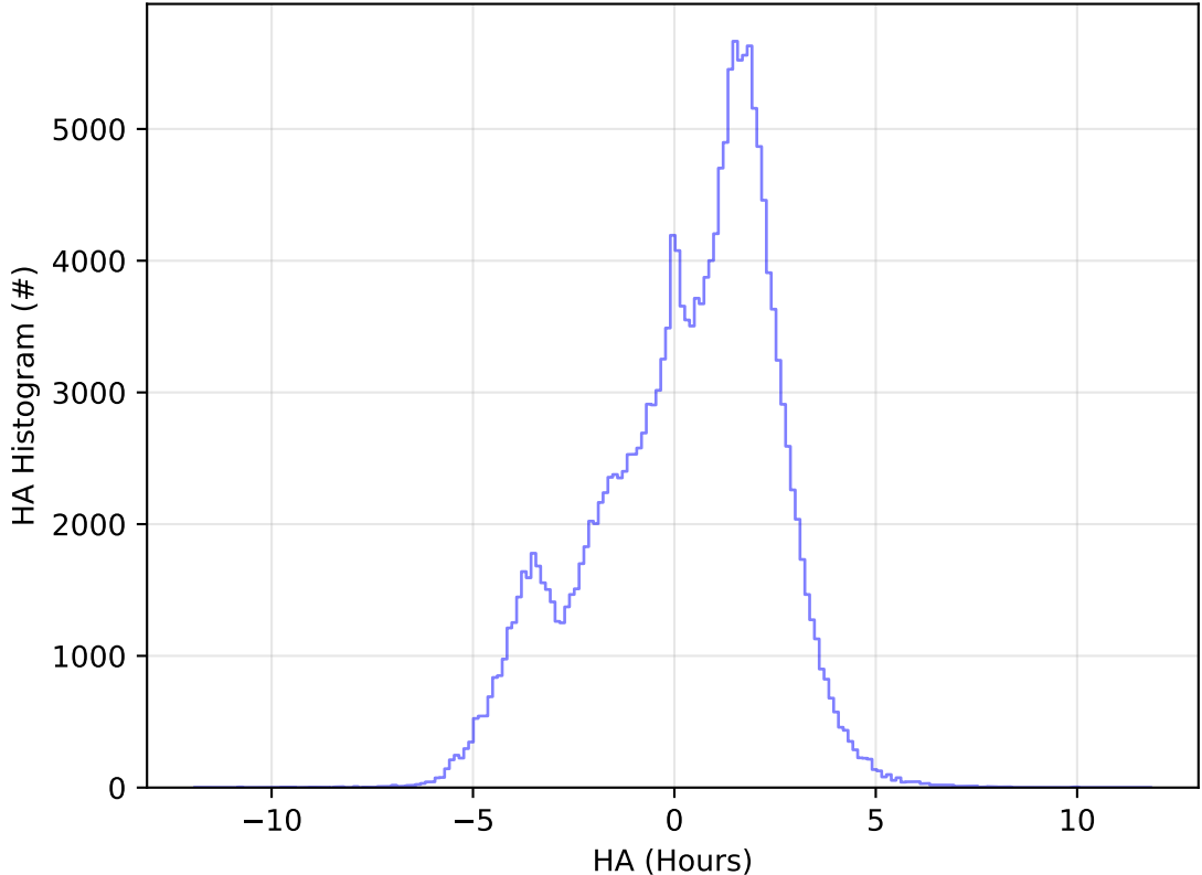
roll_uniform_early_half_accordion1_mjdp0_v3.4_10yrs WFD g band: HA Histogram
