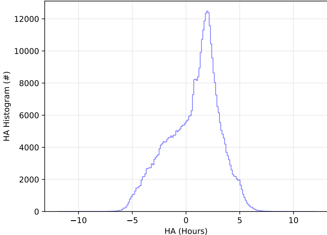
roll_uniform_early_half_accordion1_mjdp0_v3.4_10yrs All sky z band: HA Histogram
