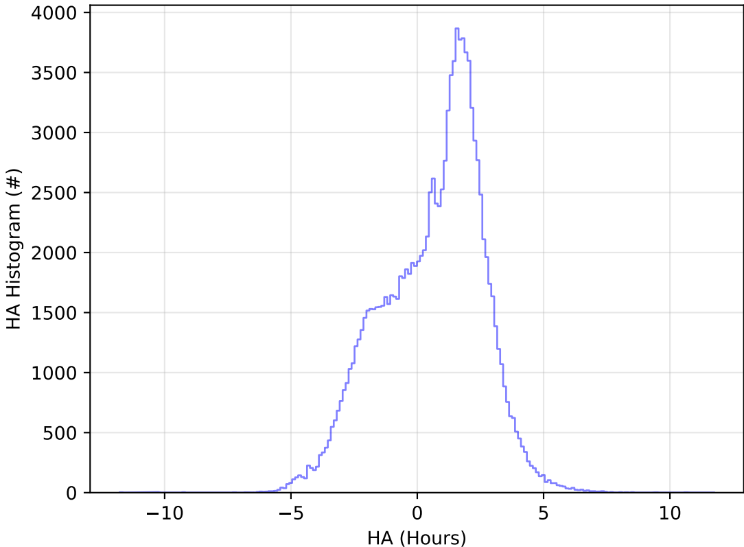
roll_uniform_early_half_accordion1_mjdp0_v3.4_10yrs All sky u band: HA Histogram
