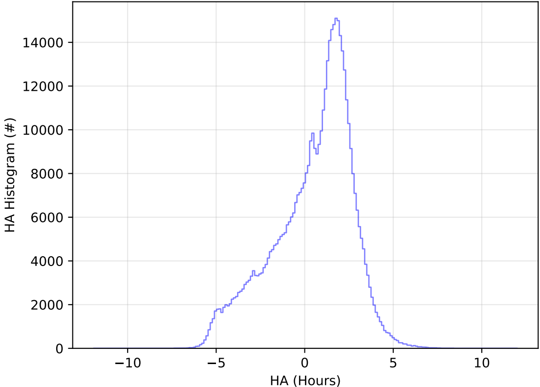
roll_uniform_early_half_accordion1_mjdp0_v3.4_10yrs All sky r band: HA Histogram
