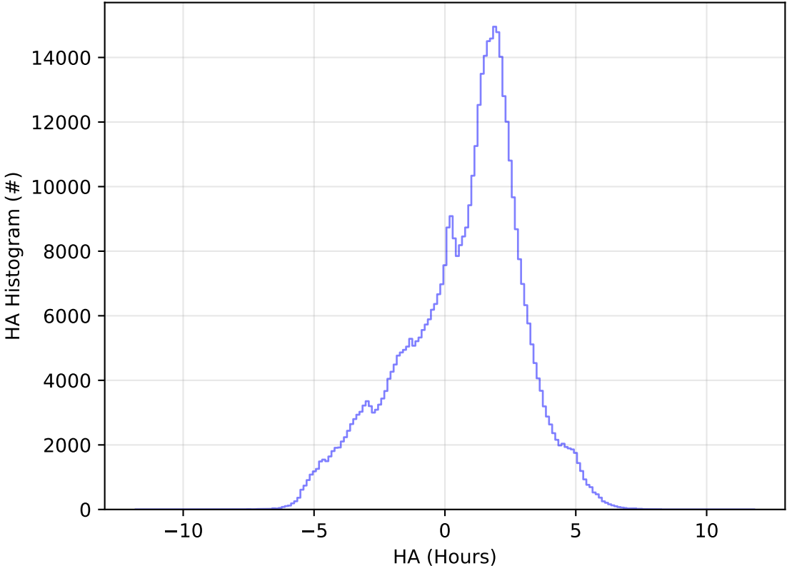
roll_uniform_early_half_accordion1_mjdp0_v3.4_10yrs All sky i band: HA Histogram
