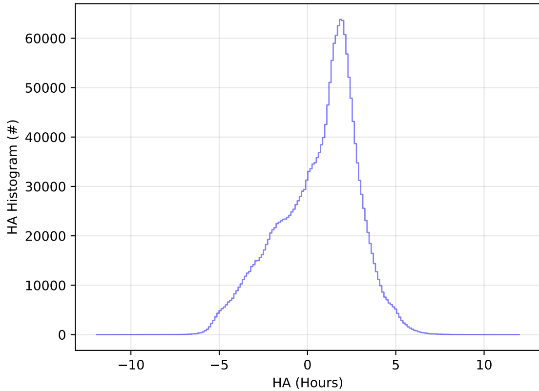
roll_uniform_early_half_accordion1_mjdp0_v3.4_10yrs All sky all bands: HA Histogram
