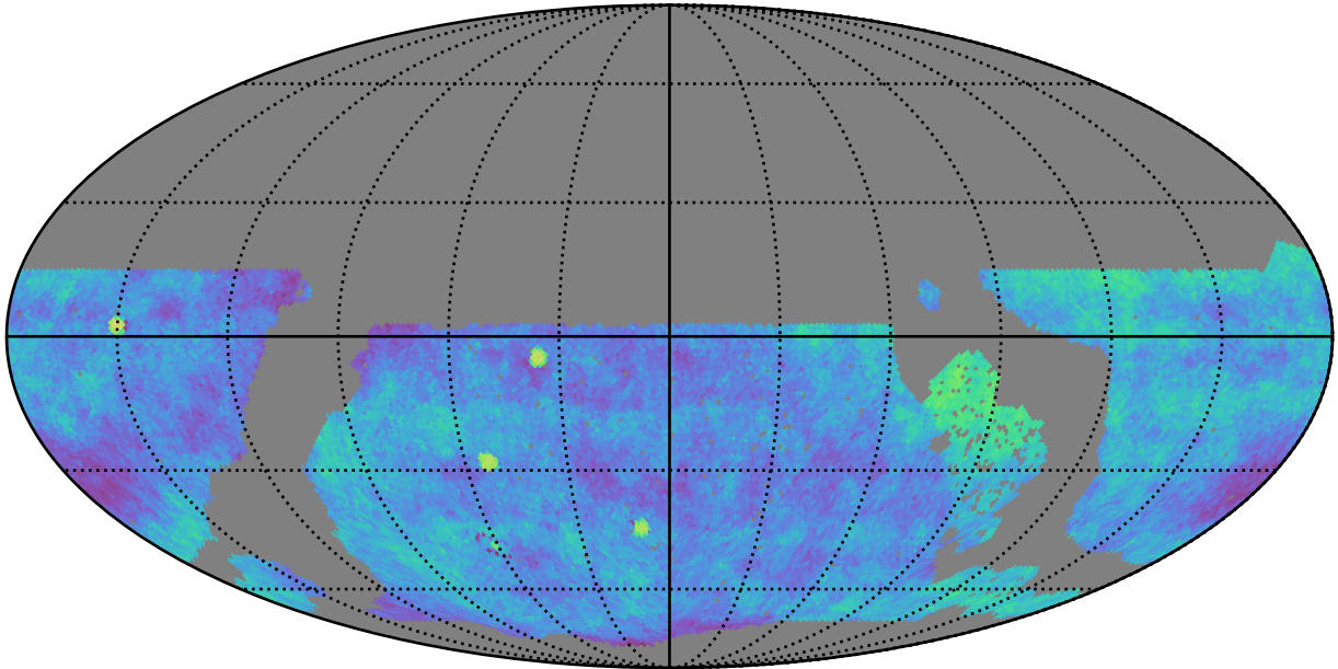
roll_uniform_early_half_accordion1_mjdp0_v3.4_10yrs gri WFD: Fraction of visits in pairs (20-90 min)
