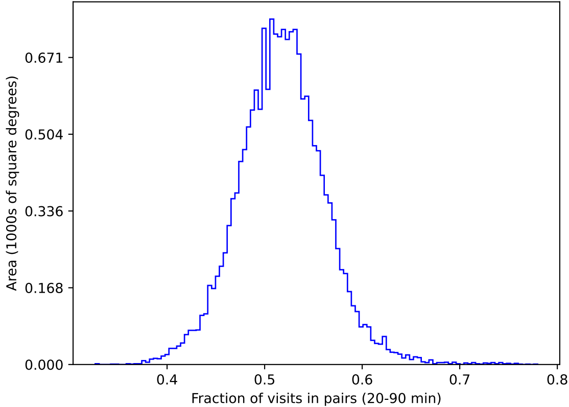
roll_uniform_early_half_accordion1_mjdp0_v3.4_10yrs gri WFD: Fraction of visits in pairs (20-90 min)
