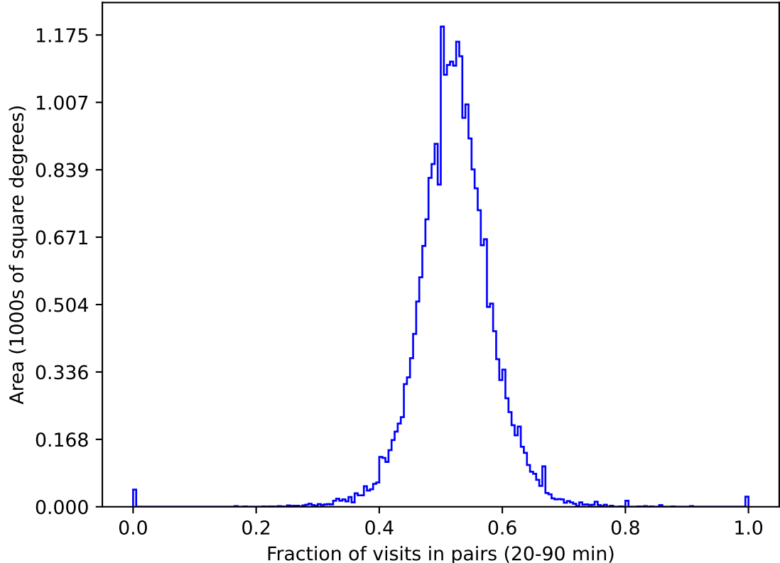
roll_uniform_early_half_accordion1_mjdp0_v3.4_10yrs gri All sky: Fraction of visits in pairs (20-90 min)
