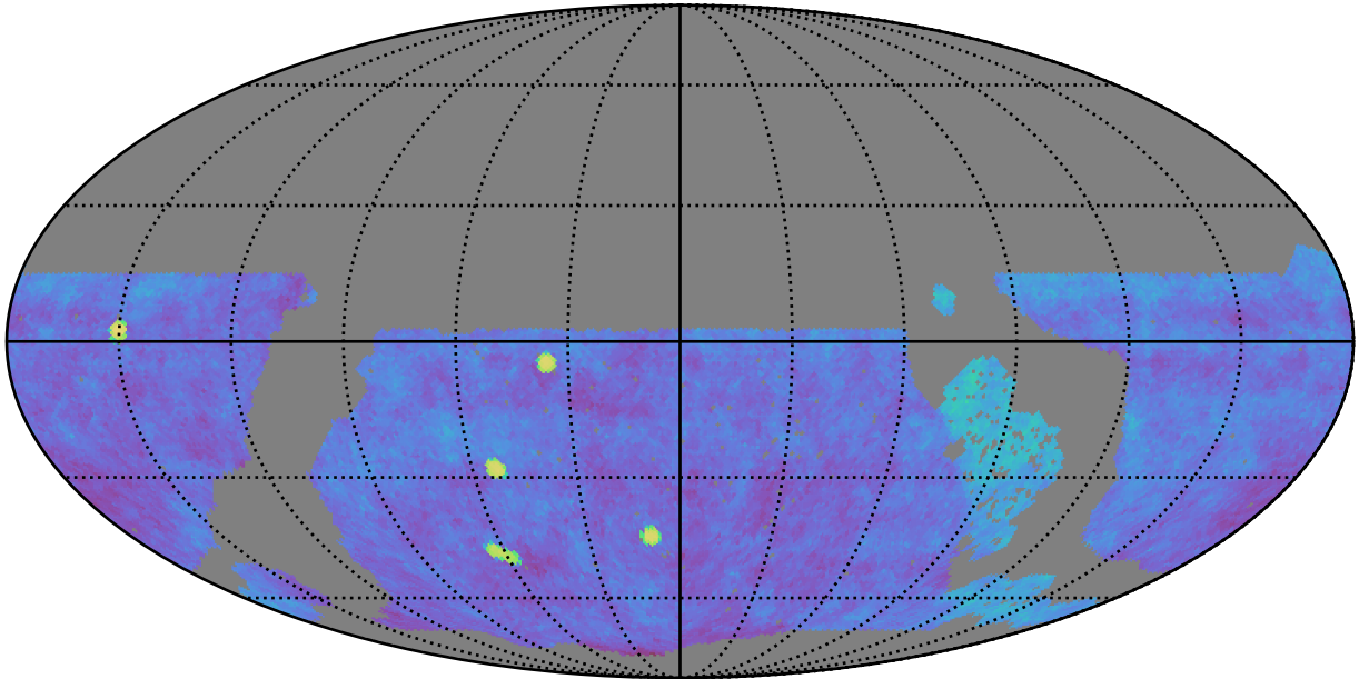
roll_uniform_early_half_accordion1_mjdp0_v3.4_10yrs gri WFD: Fraction of visits in pairs (10-60 min)
