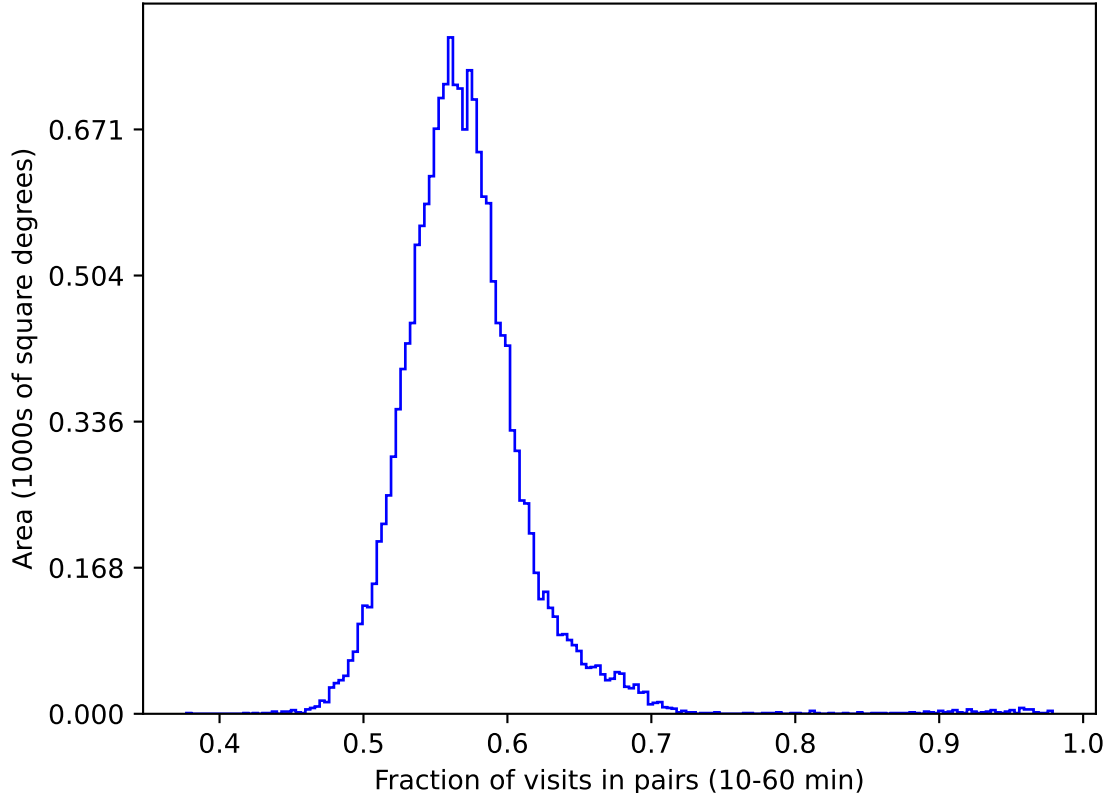
roll_uniform_early_half_accordion1_mjdp0_v3.4_10yrs gri WFD: Fraction of visits in pairs (10-60 min)
