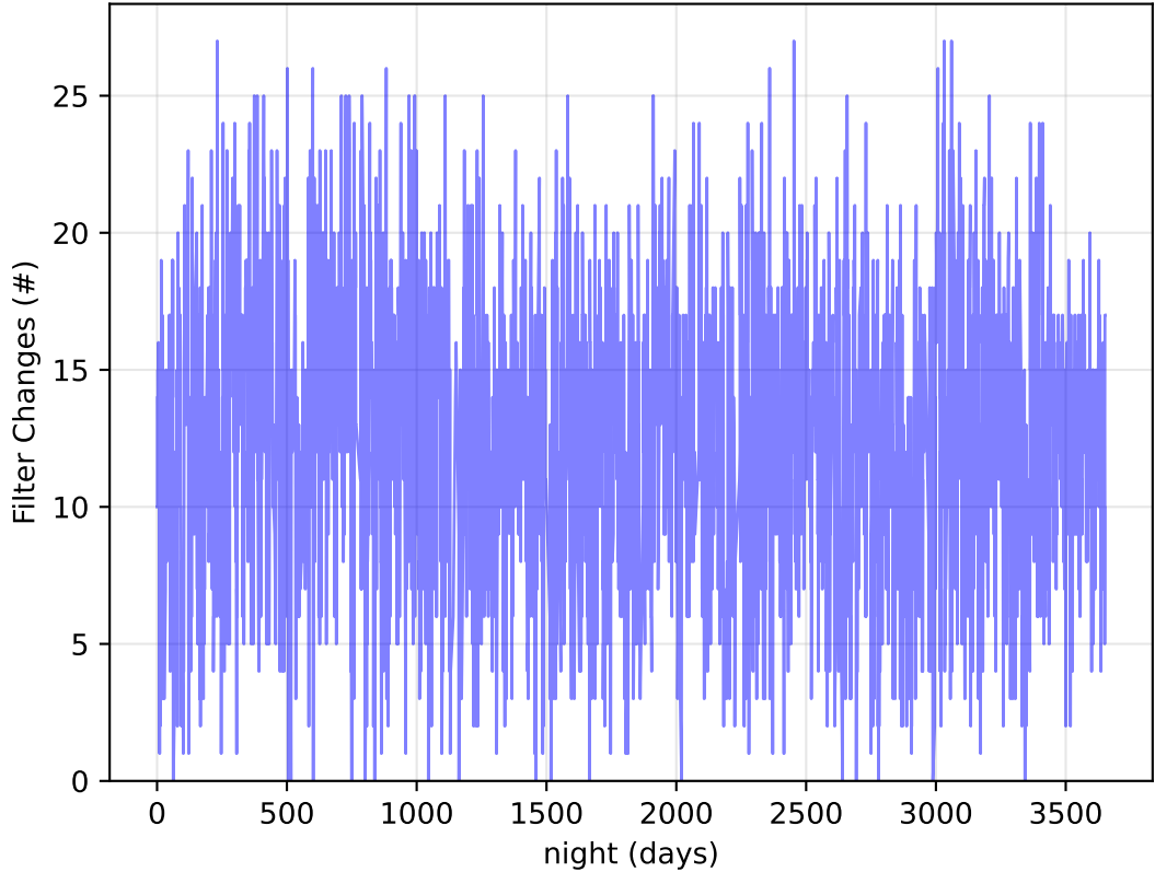
roll_uniform_early_half_accordion1_mjdp0_v3.4_10yrs Per Night: Filter Changes
