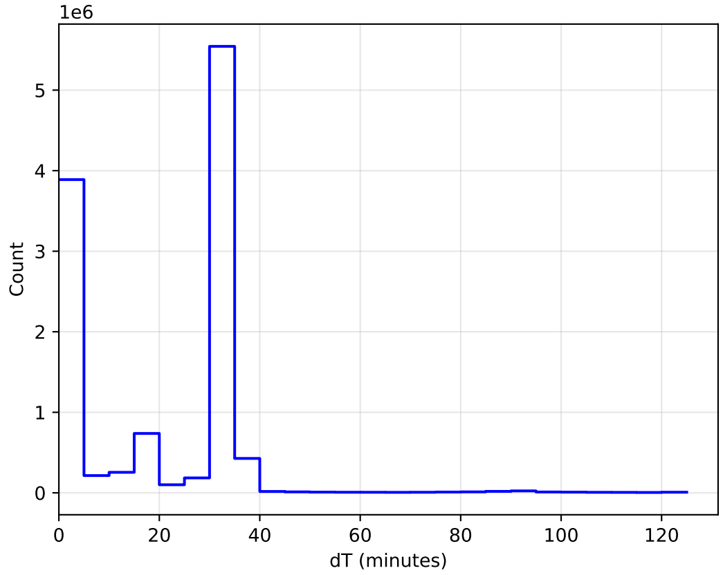
roll_uniform_early_half_accordion1_mjdp0_v3.4_10yrs WFD: DeltaT Histogram
