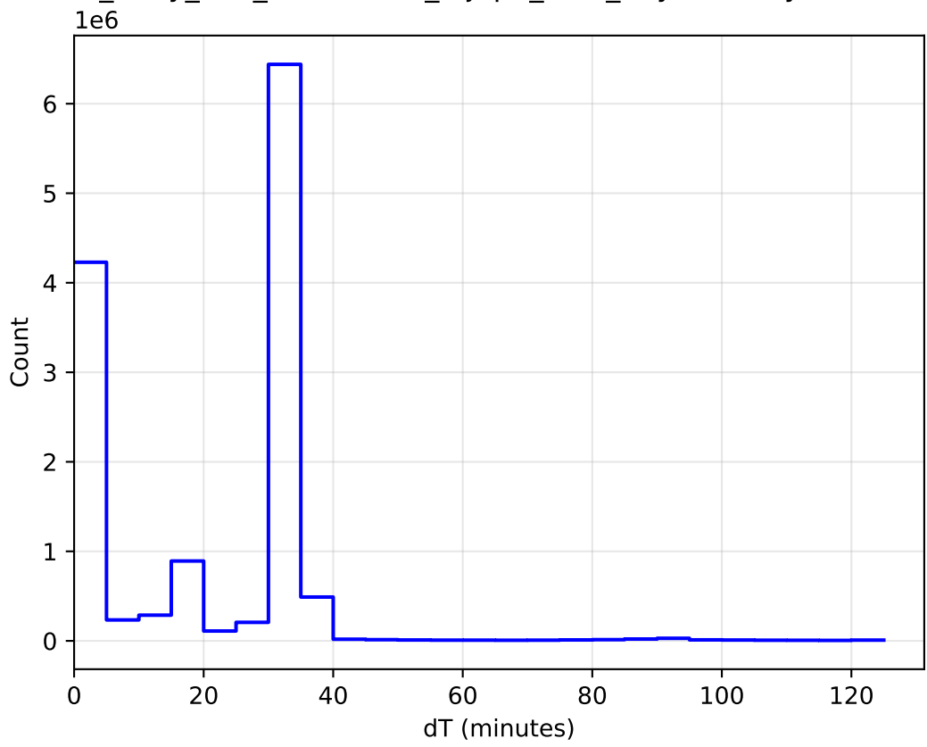
roll_uniform_early_half_accordion1_mjdp0_v3.4_10yrs All sky: DeltaT Histogram
