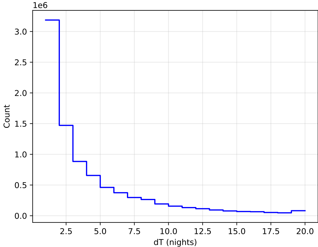
roll_uniform_early_half_accordion1_mjdp0_v3.4_10yrs All sky all bands: DeltaNight Histogram
