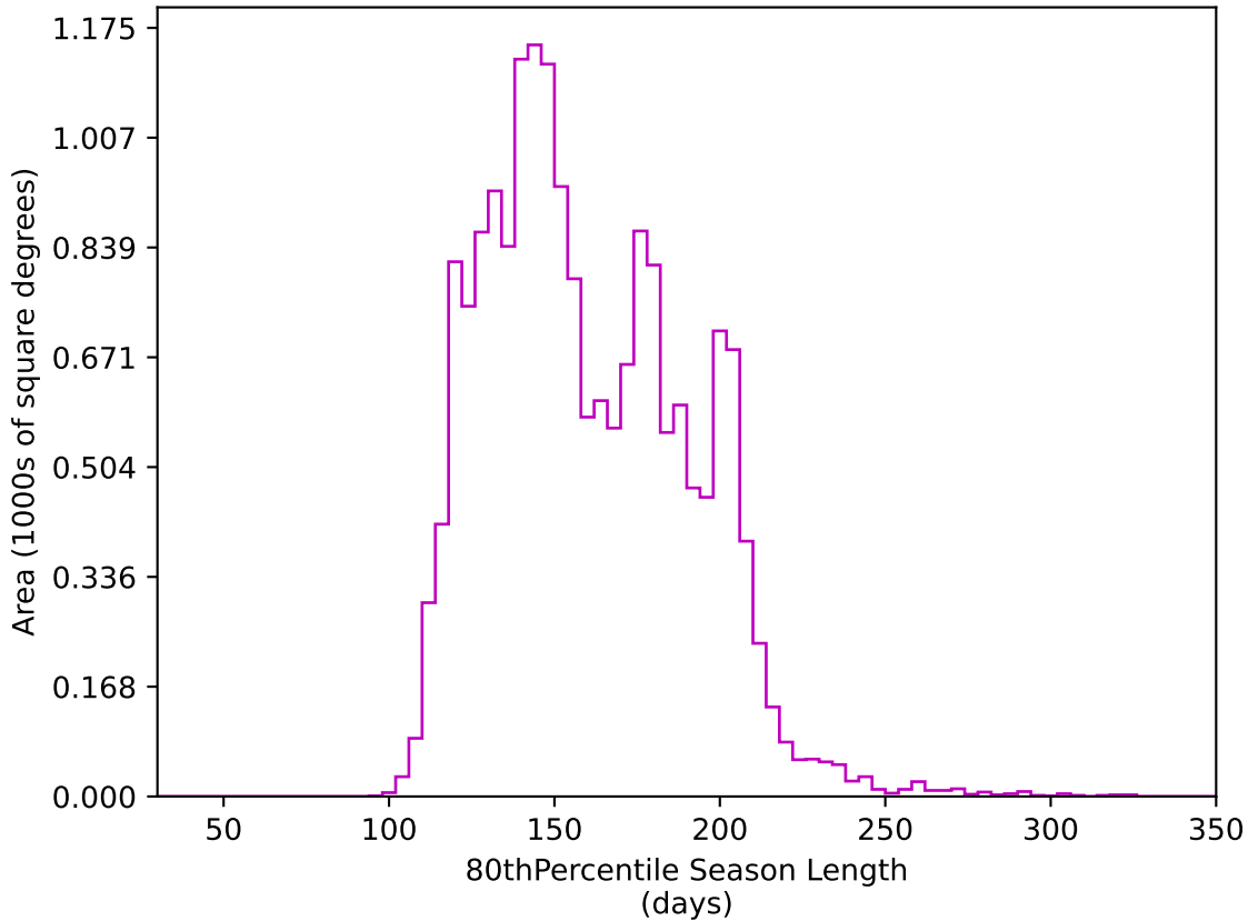
roll_uniform_early_half_accordion1_mjdp0_v3.4_10yrs WFD z band: 80thPercentile Season Length
