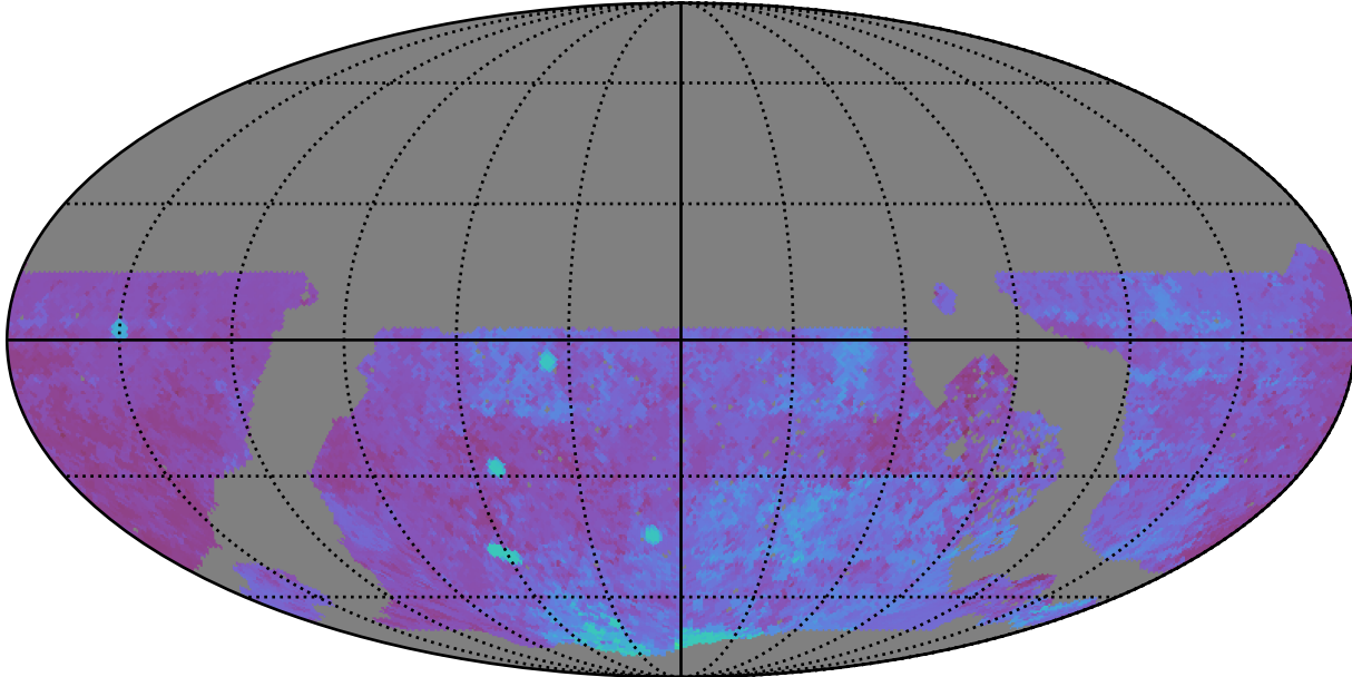
roll_uniform_early_half_accordion1_mjdp0_v3.4_10yrs WFD u band: 80thPercentile Season Length
