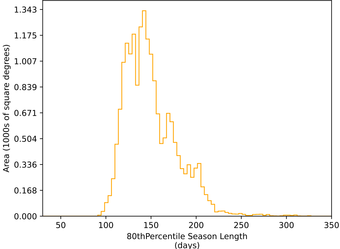
roll_uniform_early_half_accordion1_mjdp0_v3.4_10yrs WFD r band: 80thPercentile Season Length
