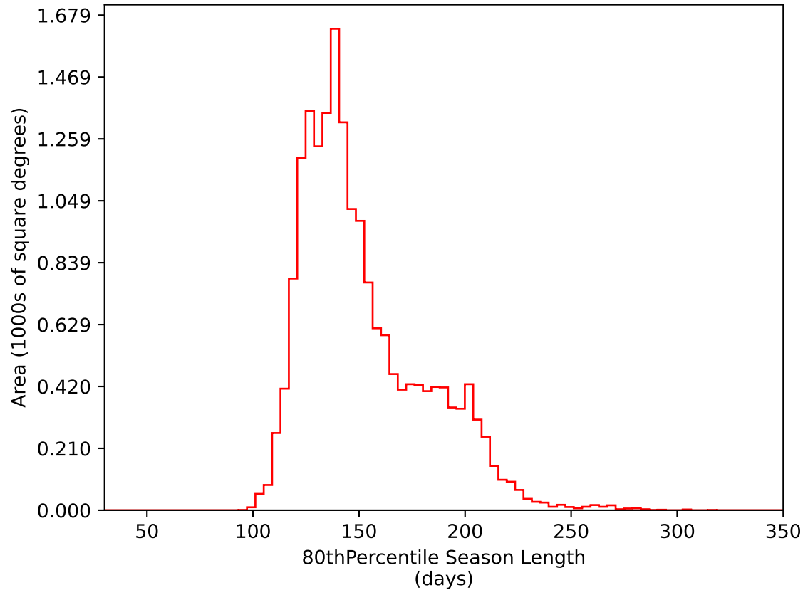
roll_uniform_early_half_accordion1_mjdp0_v3.4_10yrs WFD i band: 80thPercentile Season Length
