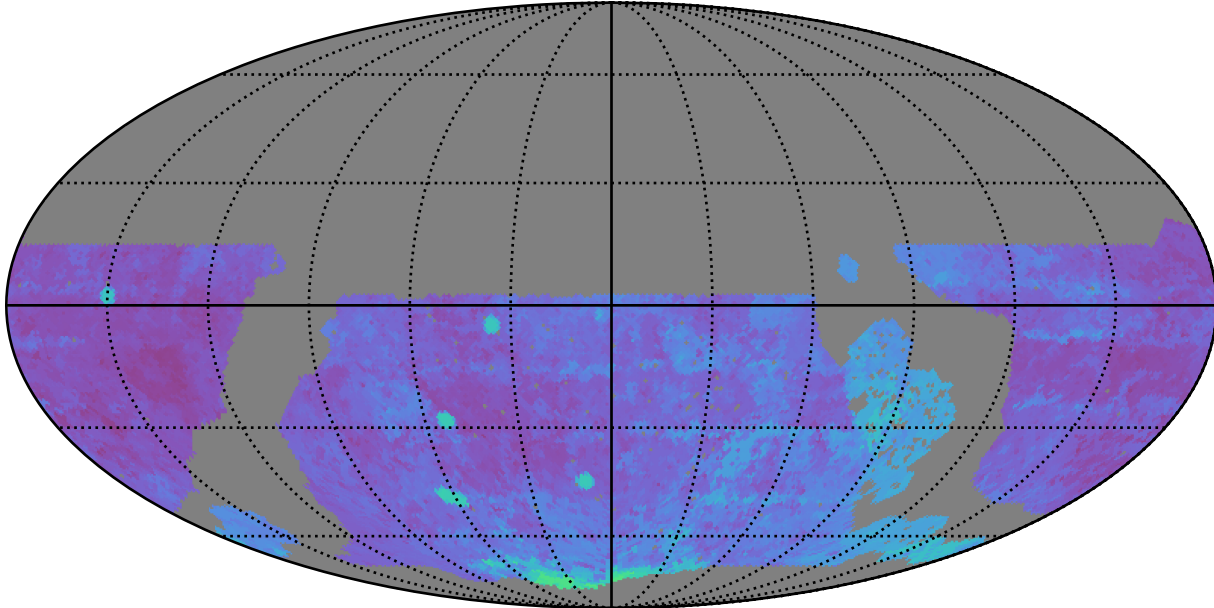
roll_uniform_early_half_accordion1_mjdp0_v3.4_10yrs WFD g band: 80thPercentile Season Length
