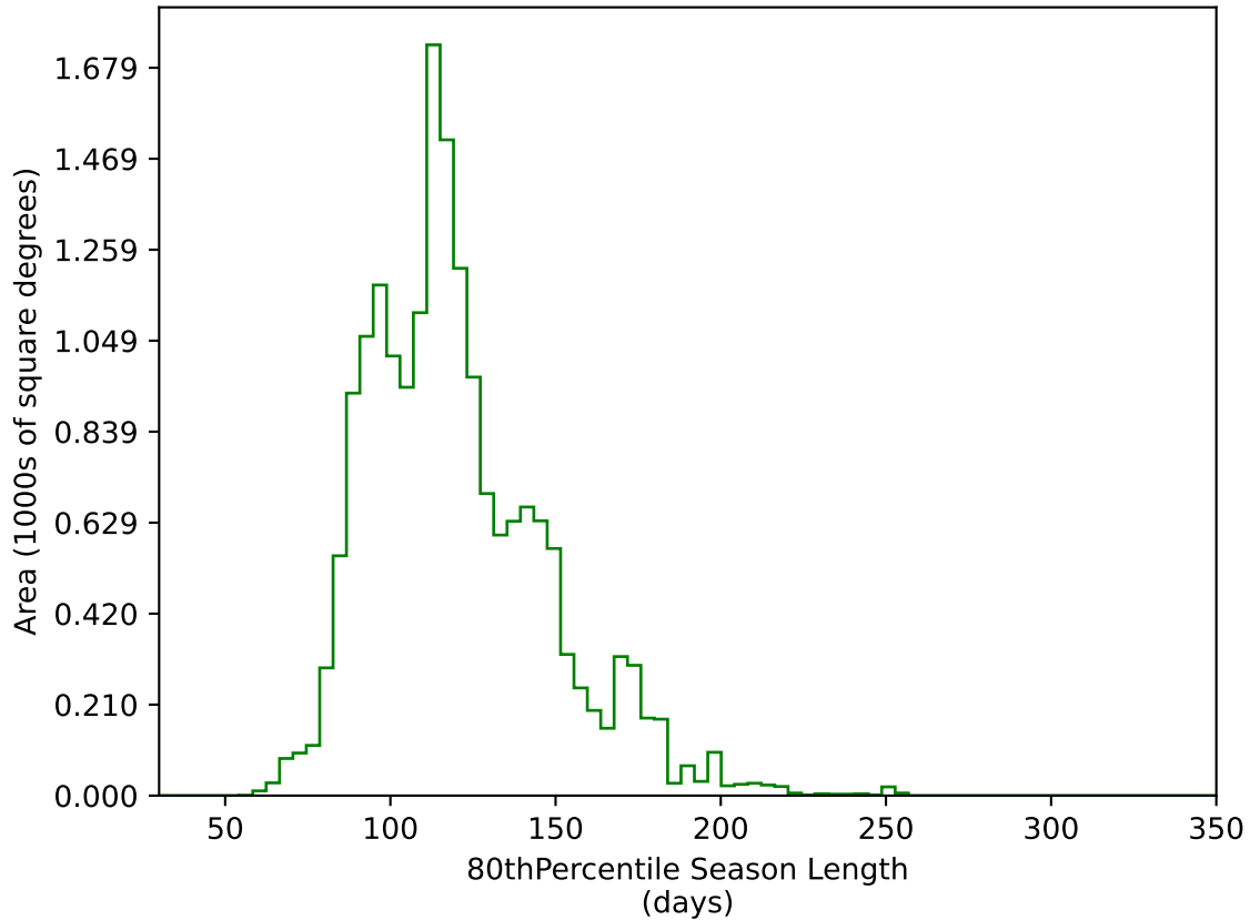
roll_uniform_early_half_accordion1_mjdp0_v3.4_10yrs WFD g band: 80thPercentile Season Length
