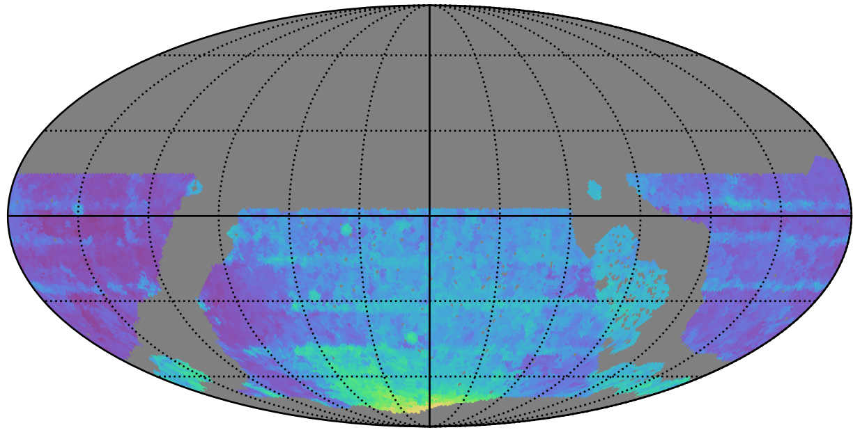
roll_uniform_early_half_accordion1_mjdp0_v3.4_10yrs WFD all bands: 80thPercentile Season Length
