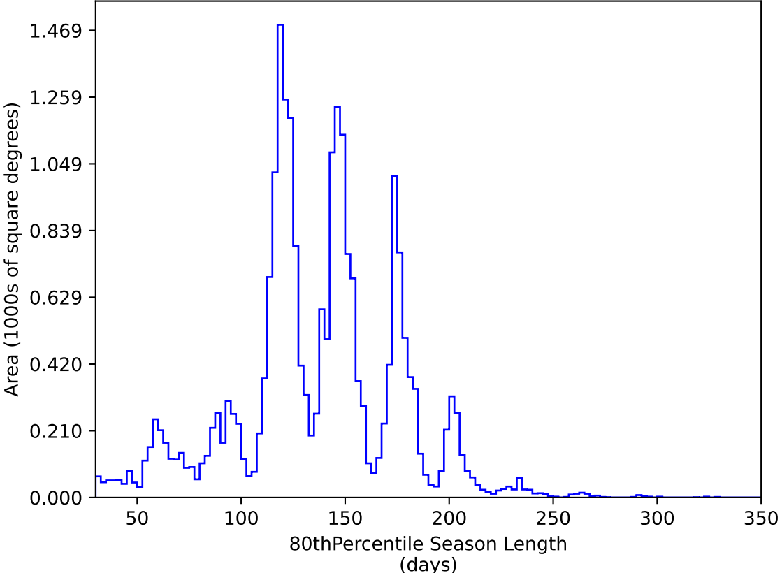
roll_uniform_early_half_accordion1_mjdp0_v3.4_10yrs All sky y band: 80thPercentile Season Length
