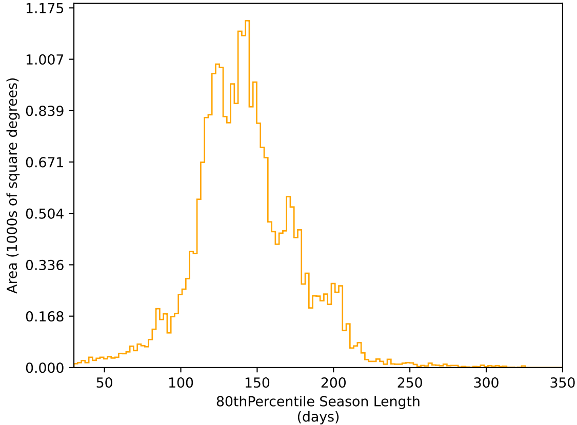
roll_uniform_early_half_accordion1_mjdp0_v3.4_10yrs All sky r band: 80thPercentile Season Length
