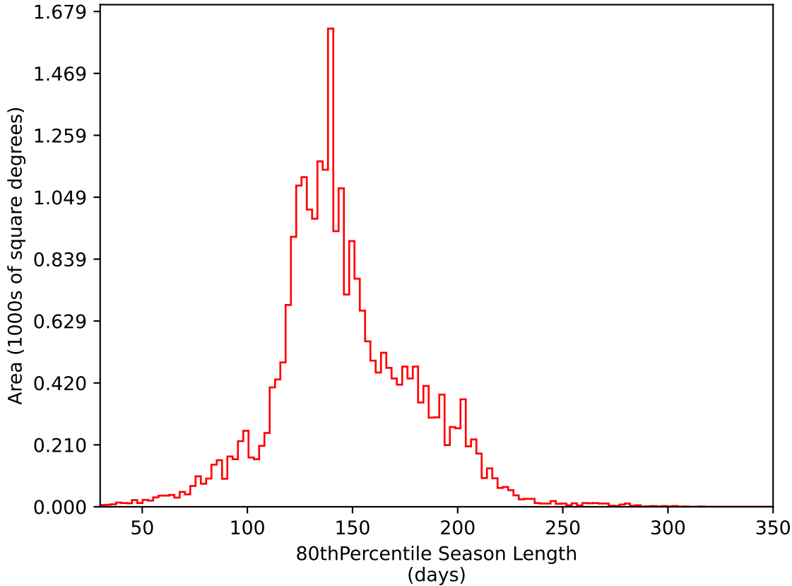
roll_uniform_early_half_accordion1_mjdp0_v3.4_10yrs All sky i band: 80thPercentile Season Length
