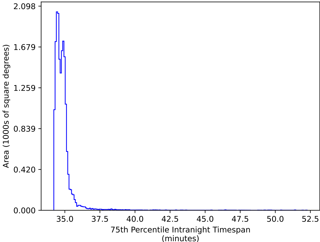
roll_uniform_early_half_accordion1_mjdp0_v3.4_10yrs WFD zy bands: 75th Percentile Intranight Timespan
