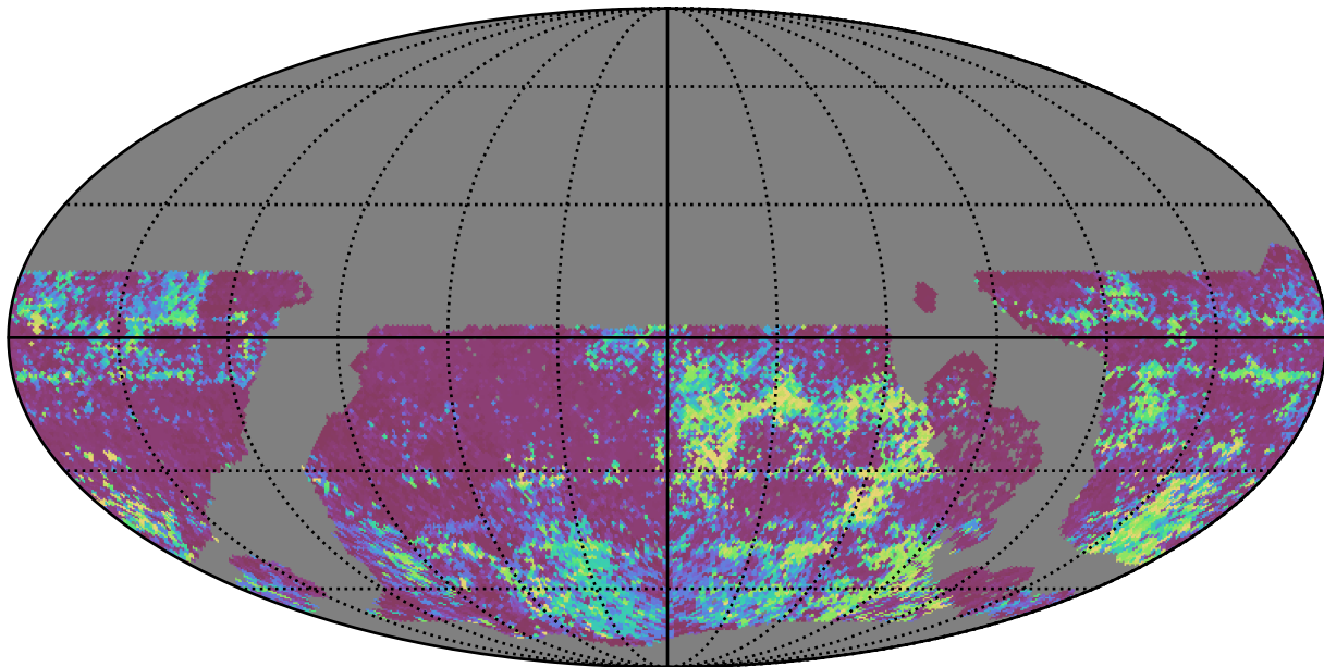
roll_uniform_early_half_accordion1_mjdp0_v3.4_10yrs WFD z band: 75th Percentile Intranight Timespan
