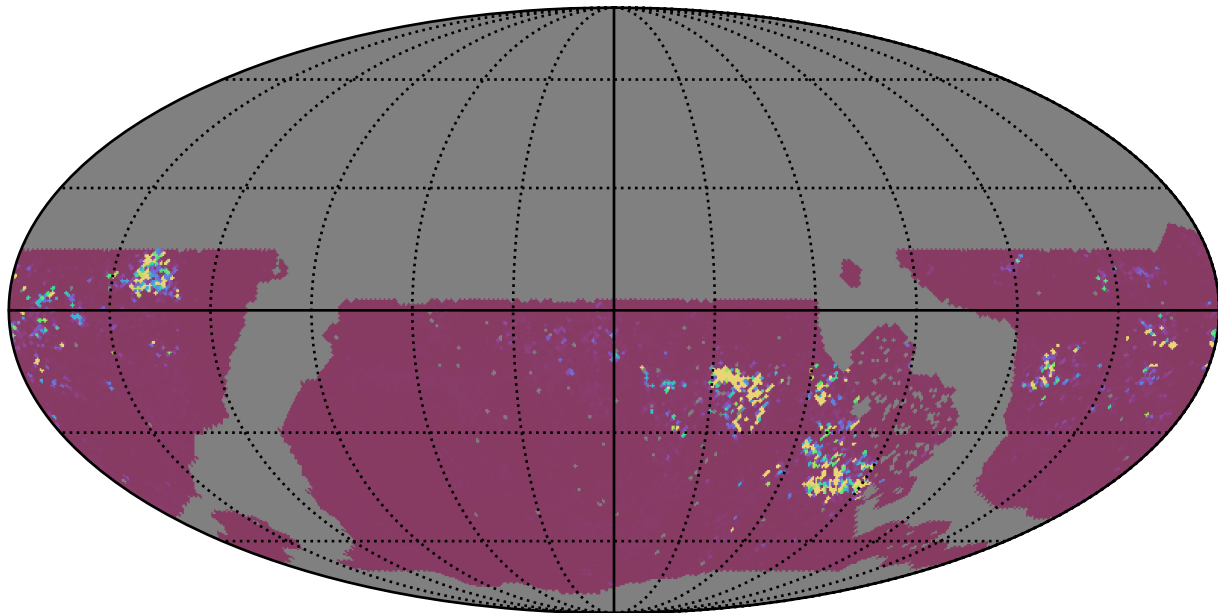
roll_uniform_early_half_accordion1_mjdp0_v3.4_10yrs WFD y band: 75th Percentile Intranight Timespan
