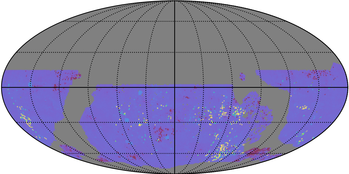
roll_uniform_early_half_accordion1_mjdp0_v3.4_10yrs WFD ug bands: 75th Percentile Intranight Timespan
