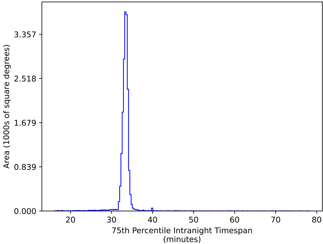
roll_uniform_early_half_accordion1_mjdp0_v3.4_10yrs WFD ug bands: 75th Percentile Intranight Timespan
